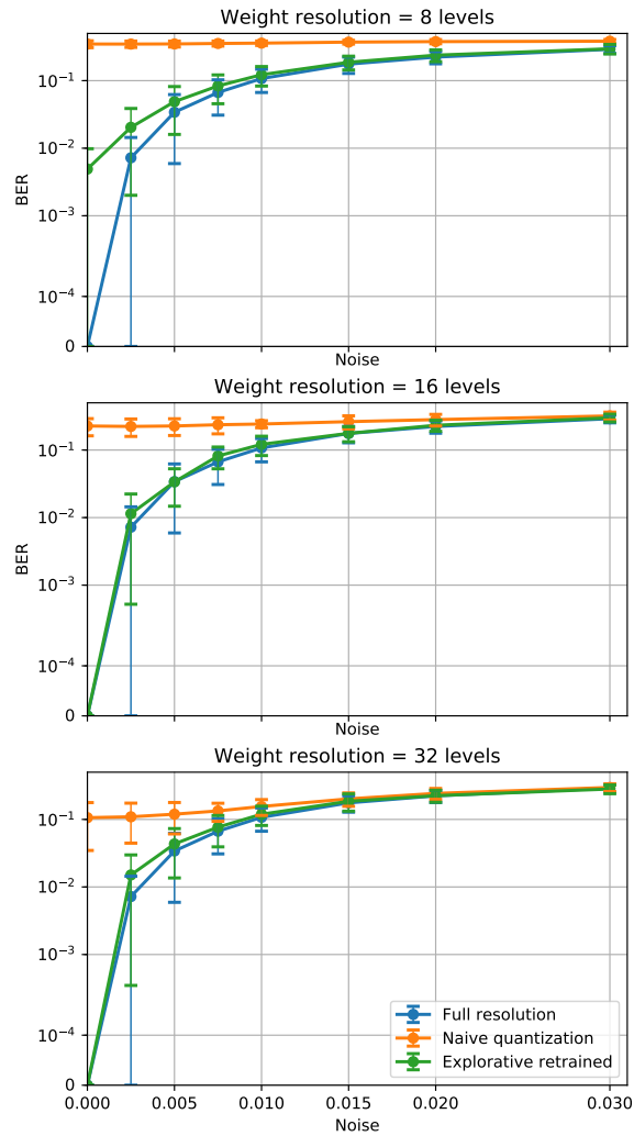
Figure 4: Performance comparison of three different weighting resolutions, 8 levels (top), 16 levels (middle), 32 levels (bottom) for the 4-bit delayed XOR task vs different noise levels. The blue curve represents the performance of full-resolution weights; the orange curve represents naive quantization weights; the green curve for explorative retrained quantization weights.
