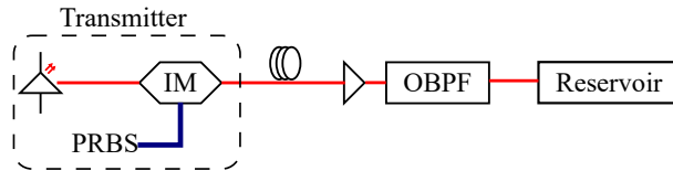
Figure 1: Schematic representation of the simulation setup to generate data for the signal equalization task. The input pseudo-random bit sequence (PRBS) signal is modulated onto a laser signal, transmitted over a fiber link, amplified and filtered, after which the field of the optical signal is saved to file to be used as input to the photonic reservoir simulation model. OBPF - Optical band pass filter.
