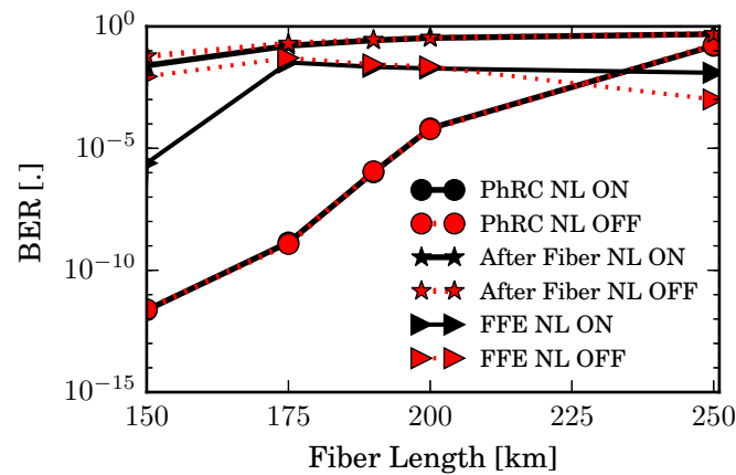
Figure 3: BER of the PhRC equalizer as compared to that of an FIR Feed Forward Equalizer (FFE) trained on the same amount of data for different fiber lengths. The launch power is set to 15 mW. NL ON- nonlinear propagation. NL OFF - nonlinear propagation is deactivated (Nonlinear Index of the fiber is set to 0).
