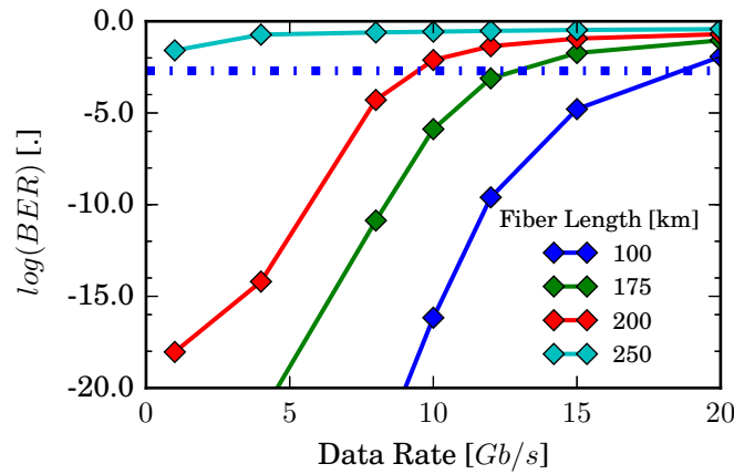
Figure 2: Error rate vs data rate for a reservoir with interconnection delay time equal to half the bit duration and latency 1 bit. A Hard Decision Forward Error Correction limit (HD-FEC limit) of 0.2 \times 10^{-2} is also shown (dashed blue line). Error free operation is possible for all error rate values below this limit.
