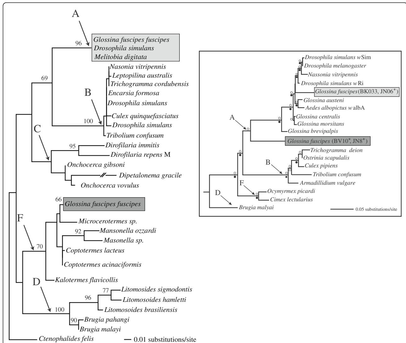
Figure 2 Rooted maximum likelihood gene tree for groEL and the tree inferred from four MLST loci (inset). Arrows point to the branch that leads to each supergroup (A-F) and are labeled accordingly for both phylogenies. Shaded clades indicate the position of G. f. fuscipes Wolbachia sequences. Light gray shading shows the position of Group 1 sequences within supergroup A. Dark gray shading shows the position of Group 2 sequences. Individual hosts that belong to each clade are shown in the additional file. (See Additional file 1: Table S1 and Figure S1). The groEL tree includes Wolbachia strains from Glossina fuscipes fuscipes and representatives from most known supergroups. For the groEL tree, the outgroup was selected arbitrarily to reflect relationships in [25]. Numbers above branches are bootstrap support percentages that are above 65%. Within supergroups for groEL , bootstrap support was below 65% and thus not reported. Inset (Upper right): A generalized version of the MLST phylogeny (See Additional file 1: Figure S1). An open circle above the branch indicates a Bayesian posterior probability of 1.0 and a closed circle below the branch is a bootstrap of 90% and above. The shaded boxes correspond to the shading of branches in the groEL phylogeny. Individuals analyzed for both groEL and MLST are indicated with an *.
