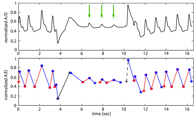
Fig. 5. When insufficient pressure was applied, pulses reappeared in the PPG during pressure application (top, arrows). The segment classification algorithm detected these pulses (bottom) and could not identify the pressure release pattern since no flat baseline was detected.
