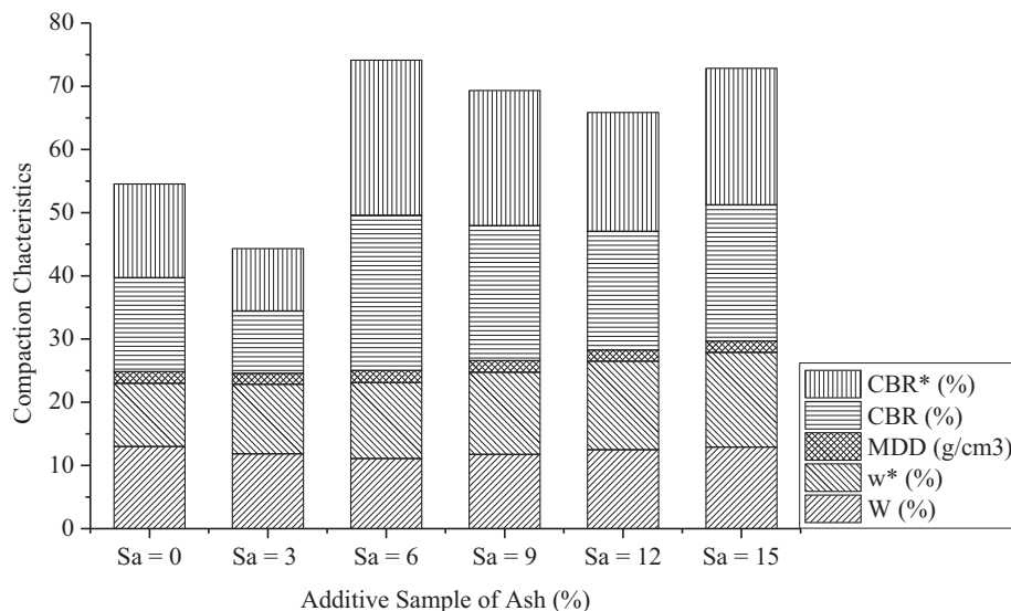
Fig. 7. California bearing ratio variables relationship model.
