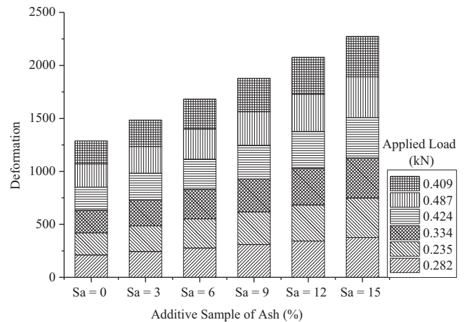
Fig. 10. Deformation of treated soils at various value of applied load.
