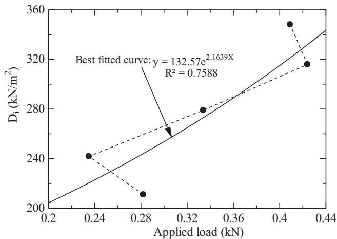
Fig. 11b. Deformation/Applied load relationship model.
