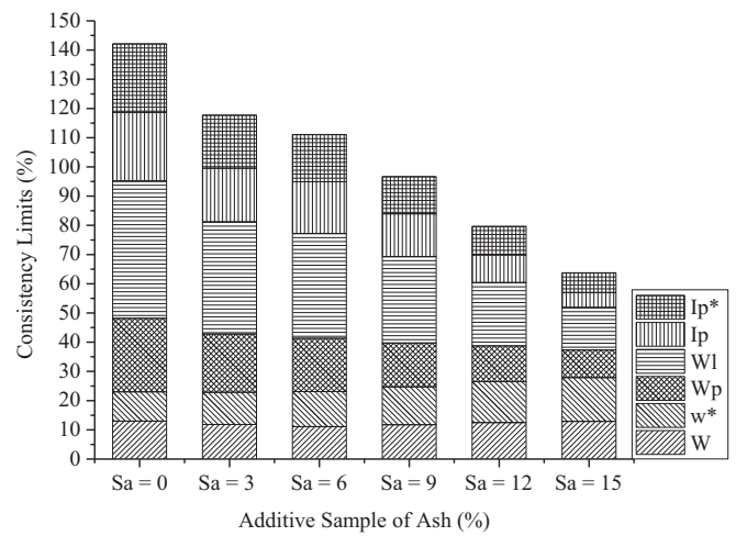
Fig. 6. Consistency limits variables relationship of model 2.
