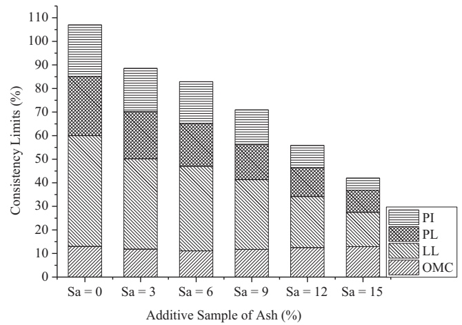
Fig. 5. Consistency behaviour of treated soils model 1.
