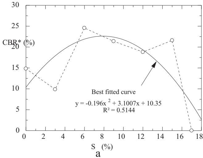
Fig. 9. CBR*/ S a relationship model.
