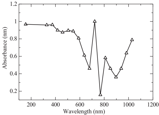
Fig. 3. Variation of absorbance against wavelength for the nanostructured palm bunch ash particles using UV/VIS spectrophotometer at 25 °C [16].
