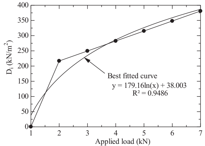
Fig. 11c. UCS Regression model relationship.
