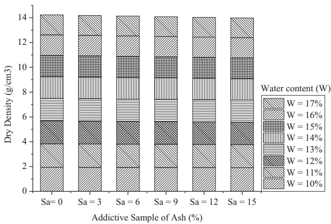
Fig. 4. Compaction variables relationship model.
