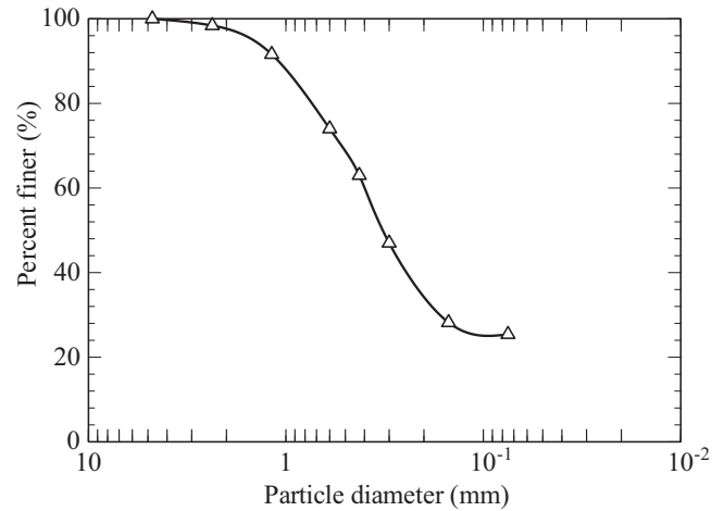
Fig. 2. Particle size distribution curve of the lateritic soil [16].
