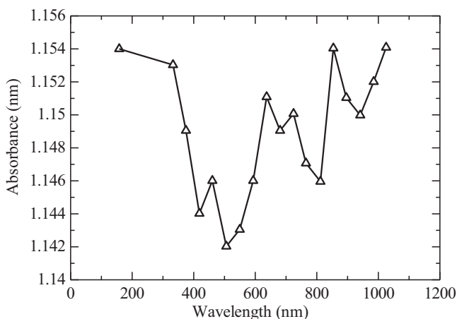
Fig. 1. Variation of absorbance against wavelength for the lateritic soil using UV/VIS spectrophotometer at 25 °C [16].
