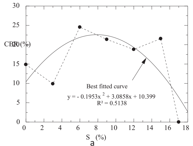
Fig. 8. CBR/ S_a relationship model.
