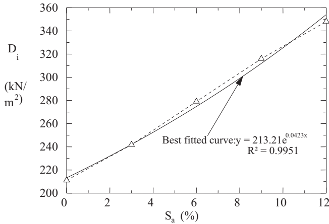
Fig. 11a. Deformation/ S_a relationship model.
