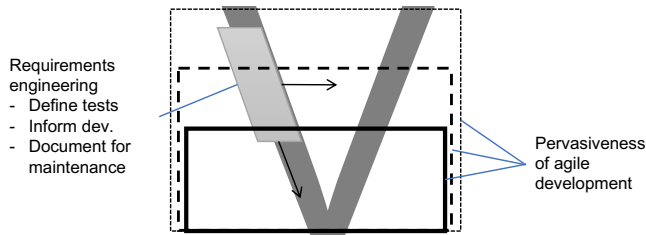
Figure 3: Different scopes of agile development within system development and a typical V model. (Light grey box denotes RE, arrows indicate how requirements are used for informing developers about what to implement, testers about what to test, and for documenting the system for maintenance. Three black boxes show the different agile scopes discussed in this case study.)
