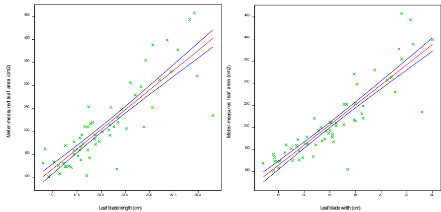
Fig. 2. The relationship between the meter measure leaf area and leaf blade length (left) and leaf blade width (right) for pure lines.
