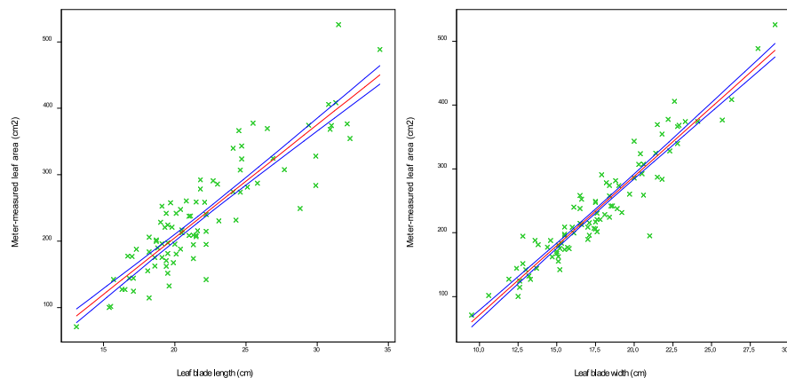
Fig. 3. The relationship between the meter measure leaf area and leaf blade length (left) and leaf blade width (right) for hybrids.
