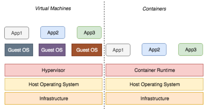
Figure 1: Difference between Virtual Machines and Containers
