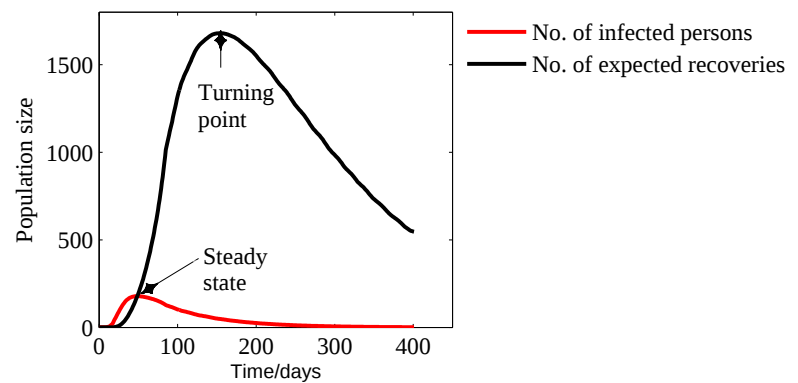
Fig. 5. Model (1) simulations for time series projection for the infected and expected recovered persons from COVID-19 in the presence of prevention and control measures.
