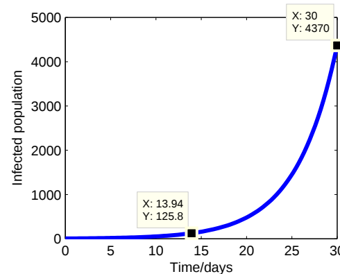
Fig. 2. The exponential projection of the number of infected individuals due to COVID-19 in Uganda without interventions (March, 2020)
