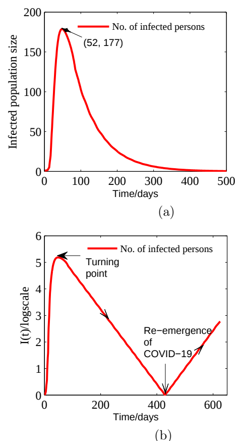
Fig. 6. (a) The number of infected persons as a function of time to linear scale. (b) The number of infected persons as a function of time to logarithm scale for R_{n0} = 0.46
