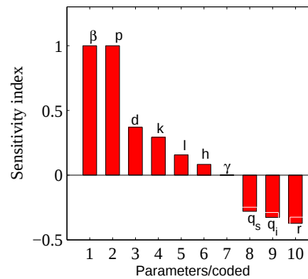
Fig. 4. Sensitivity analysis of different parameters on the basic reproduction number R_{n0}
