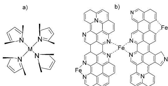
Figure 2. Active sites of a) M-N_4/C and b) Fe-N_2/C and Fe-N_{2+2}/C in M-N_x/C catalysts. Redrawn from Refs. [45] and [115], respectively, with some minor modifications, with permission from the ACS and the AAAS.
