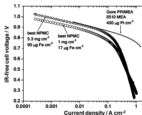
Figure 5. Polarization curves of a \text{H}_2/\text{O}_2 fuel cell with the cathode based on a \text{Fe-N}_x/\text{C} catalyst at a loading of 1 \text{ mg cm}^{-2} (circles) and 5.3 \text{ mg cm}^{-2} (stars). Also included is a ready-to-use Gore PRIMEA membrane electrode assembly (MEA; W. L. Gore & Associates) with ca. 0.4 \text{ mg Pt cm}^{-2} at the cathode and anode. Reproduced from Ref. [107] with permission from the AAAS.
