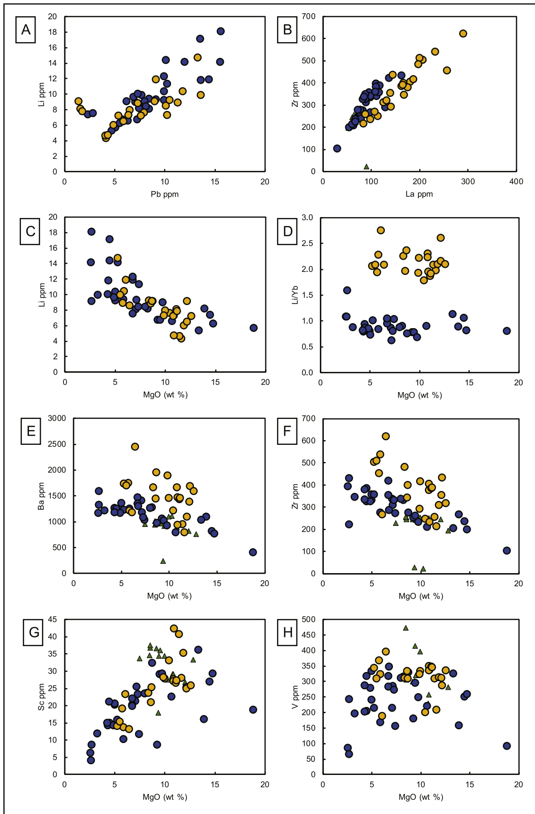
Fig. 4. Incompatible and compatible trace element variations relative to MgO in Bufumbira, Toro Ankle, and PKB lavas. These data are consistent with removal of olivine and clinopyroxene from parental melts, and with some olivine and clinopyroxene accumulation in the most MgO-rich melts.
