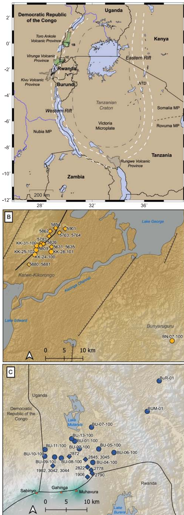
Fig. 1. A) Map of Western Rift volcanic provinces, Tanzanian Craton, and major structures of the Western and Eastern Rifts of the EARS. Microplate names and locations from Stamps et al. (2008). Western Rift volcanic province (VP) areas after Barker and Nixon (1989), Furman (1995), Pouclet et al. (2016). NTD = Northern Tanzania Divergence. B) sample locations for Katwe-Kikorongo samples; C) sample locations for Bufumbira samples; diamonds indicate Combe collection samples (Holmes and Harwood, 1932, 1937); circles indicate samples collected by the authors. Data sources and mapping tools: (MacGregor, 2015); Wessel et al., 2019); NASA SRTM). Map produced using QGIS and GMT software.
