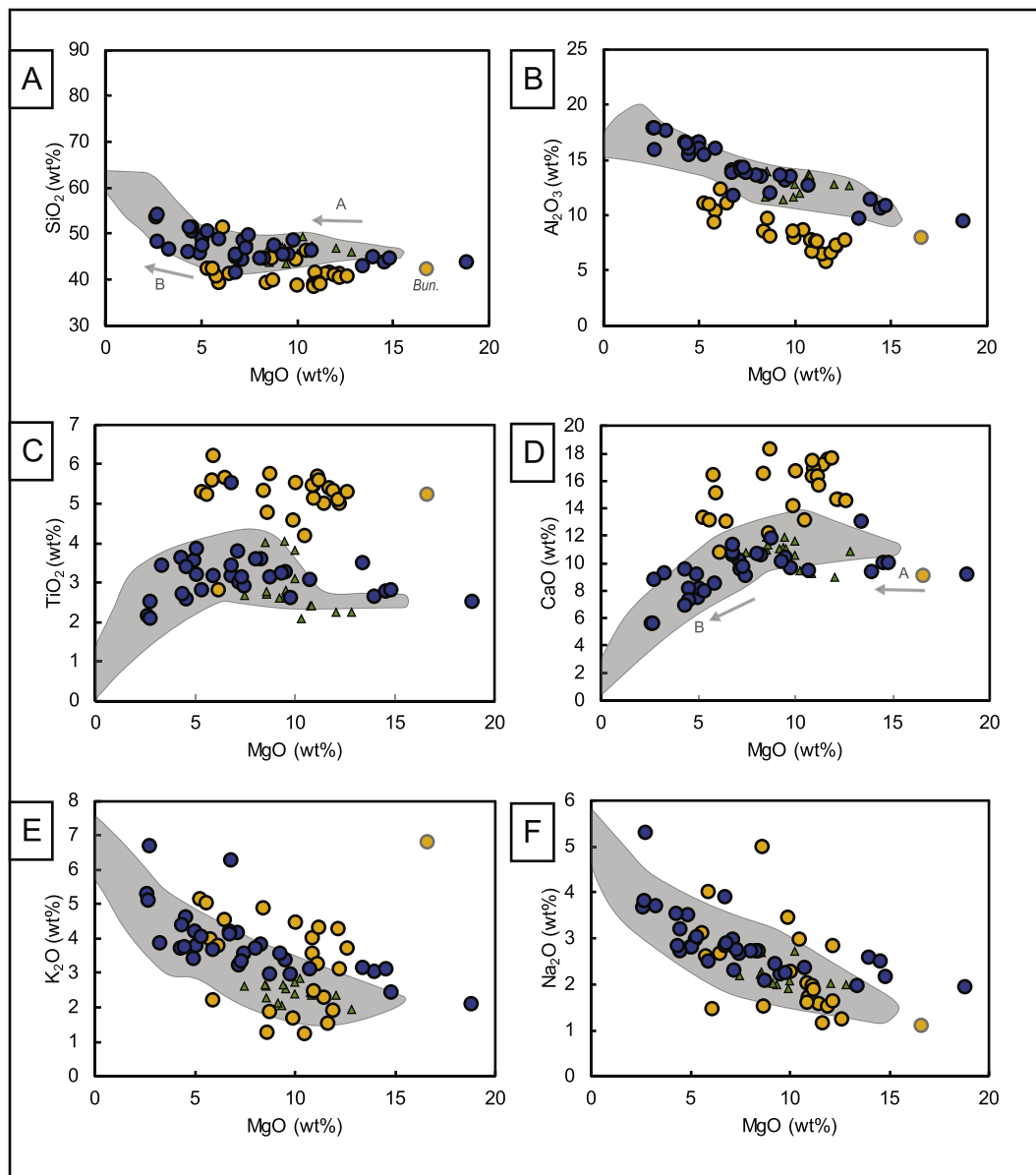
Fig. 3. Major element variation diagrams for Katwe-Kikorongo, Bunyaruguru, Bufumbira, and Karisimbi PKB lavas. Lavas from the other Virunga volcanoes are represented by gray fields. Symbols and data sources same as Fig. 2. Approximate fractionation trends are shown for primitive lavas >8% MgO (trend A; high-Mg olivine and clinopyroxene) and more evolved compositions <8% MgO (trend B; lower-Mg olivine and clinopyroxene, high-An plagioclase, ilmenite, spinel, rutile and magnetite) on selected plots (see Section 5.1 for discussion).
