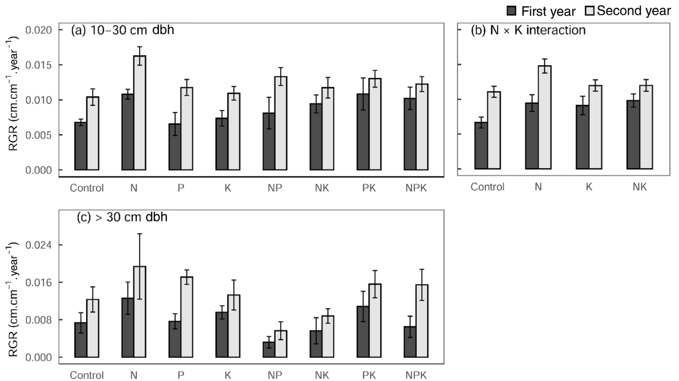
FIGURE 2 Relative growth rate (RGR; mean \pm SE) responses of different tree size classes to nutrient additions for trees \geq 10 cm diameter at breast height (dbh). Census intervals for 2018–2019 and 2019–2020 are reported as first and second years of growth, respectively. (a) RGR of trees 10–30 cm dbh, where we found a positive RGR response to N additions in the second year ( F_{1,24} = 4.76 , p = 0.039 ; n = 4 plots with full factorial ANOVA). (b) Illustration of a negative N \times K interaction (for trees 10–30 cm dbh in the second year) with RGR enhanced in the +N treatment but not in the +NK treatment ( F_{1,24} = 4.71 , p = 0.040 ; n = 8 plots; full factorial ANOVA). (c) A positive response to N \times P \times K interaction for trees \geq 30 cm dbh was found in the second year ( F_{1,24} = 5.56 , p = 0.027 ; n = 4 plots with full factorial ANOVA)
