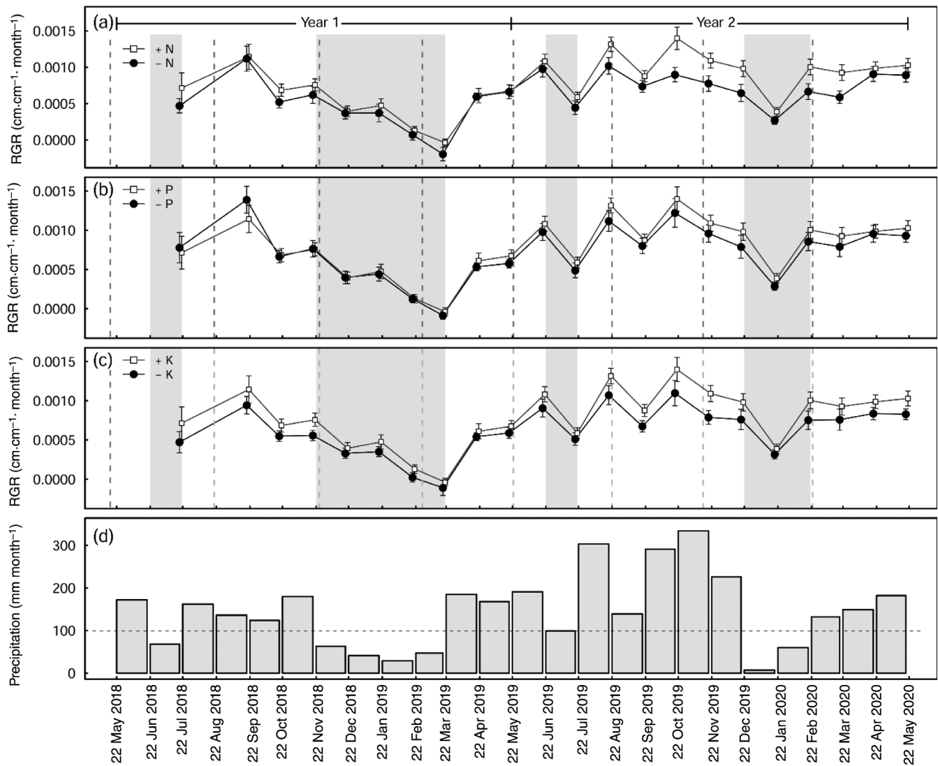
FIGURE 1 Relative growth rate (RGR) responses of trees 10–30 cm diameter at breast height (dbh; 82% of 656 trees on which dendrometer bands were installed) to nitrogen (N), phosphorus (P), and potassium (K) additions. Presented are (a) pooled +N (N, N + P, N + K, and N + P + K) and –N (control, K, P, and P + K), (b) +P (P, N + P, P + K, and N + P + K) and –P (control, N, K and N + K), (c) +K (K, P + K, N + K and N + P + K) and –K (control, N, P and N + P), and (d) monthly precipitation. Error bars are standard errors of the mean for each treatment aggregation, n = 16 plots. Statistical analysis was based on the eight treatments in the full factorial NPK design where the main effect of N additions was found in the second year (linear mixed-effects model; F_{1,24} = 6.14 , p = 0.021 ). Dotted vertical lines correspond to dates of nutrient additions; gray shades represent dry months (<100 mm/month precipitation, shown by the horizontal dotted line in panel d)
