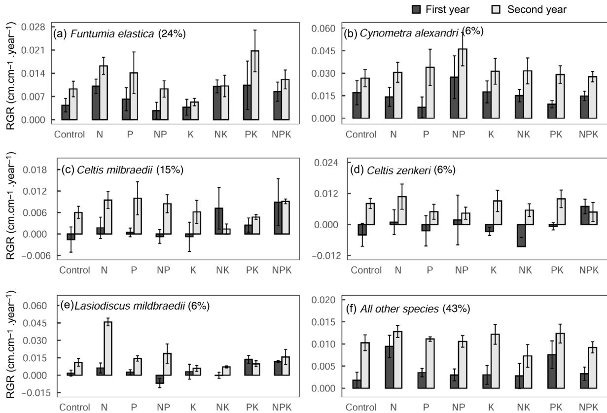
FIGURE 3 Relative growth rate (RGR; mean ± SE) response of different tree species (a–e; representing 57% of tree abundance and all other species combined [f]) to nutrient additions, for trees ≥10 cm diameter at breast height (dbh). Census intervals for 2018–2019 and 2019–2020 are reported as first and second years of growth. All panels present the eight treatments of the full factorial NPK design. Bars represent the RGR of at least three replicate plots per treatment. For Funtumia elastica in the second year, the N × P interaction was significantly negative with greater growth in the +N, +P, +NK, and +PK treatments and lower growth in the +NP and +NPK treatments (panel a; F_{1,24} = 5.45, p = 0.028 ). For Lasiodiscus mildbraedii (panel e), N addition increased RGR significantly in the second year ( F_{1,20} = 8.06, p = 0.010 ) and K addition reduced RGR in both years ( F_{1,20} = 5.68, 13.03; p = 0.027, 0.002 ); however, the P × K interaction was also significant and positive in both years with greater RGR in the +PK and +NPK treatments ( F_{1,20} = 10.12, 5.06; p = 0.005, 0.036 ). For all other species, the P × K interaction was significant and positive in the first year, with greater RGR in the +PK and +NPK treatments and lower RGR in the +P, +K, +NP, and +NK treatments (panel f; F_{1,24} = 5.12, p = 0.033 )
