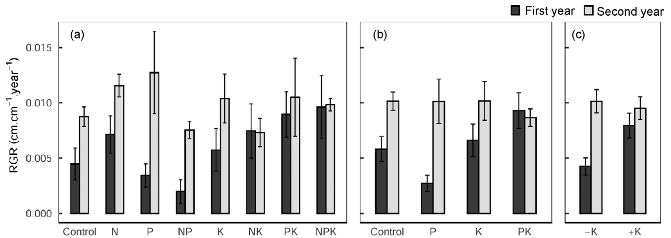
FIGURE 4 Relative growth rate (RGR; mean \pm SE) responses of semi-deciduous trees ( \geq 10 cm diameter at breast height) to nutrient additions. Census intervals for 2018–2019 and 2019–2020 are reported as first and second years of growth. (a) The eight treatments of the full factorial NPK design. To the right are the four treatments with K additions, illustrating the positive effect of K additions on RGR in the first year ( F_{1,24} = 7.48 , p = 0.012 ). (b) A significant, positive P \times K interaction effect in the first year ( F_{1,24} = 4.80 , p = 0.042 ). Sample size is eight plots for each bar: Control (control, +N), P (+P, +NP), K (+K, +NK) and PK (+PK, +NPK). (c) The significant effect of K additions for the first year. Treatments without added K (control, +N, +P, +NP) are pooled (denoted –K on the horizontal axis) with the appropriate treatments with K (+K, +NK, +PK, +NPK); thus, the sample size is 16 plots for each bar
