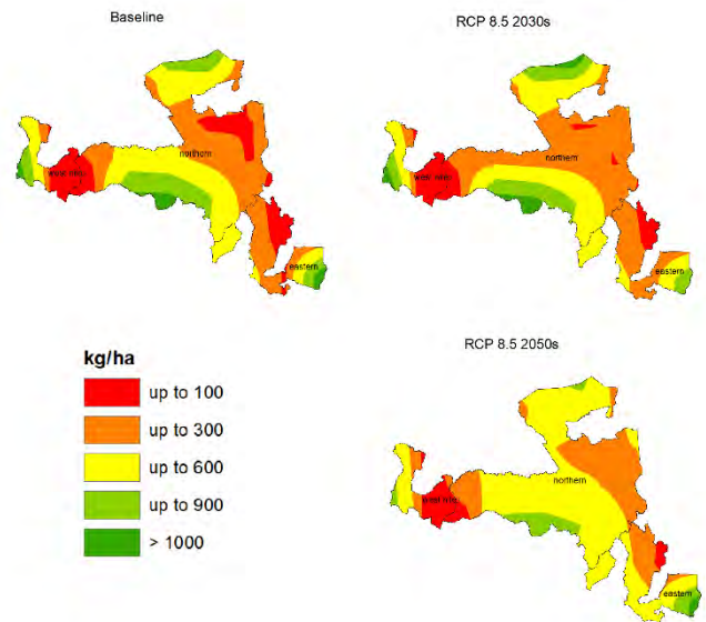
Figure 7. Modelled sunflower yields under current and future climates (RCP8.5)
