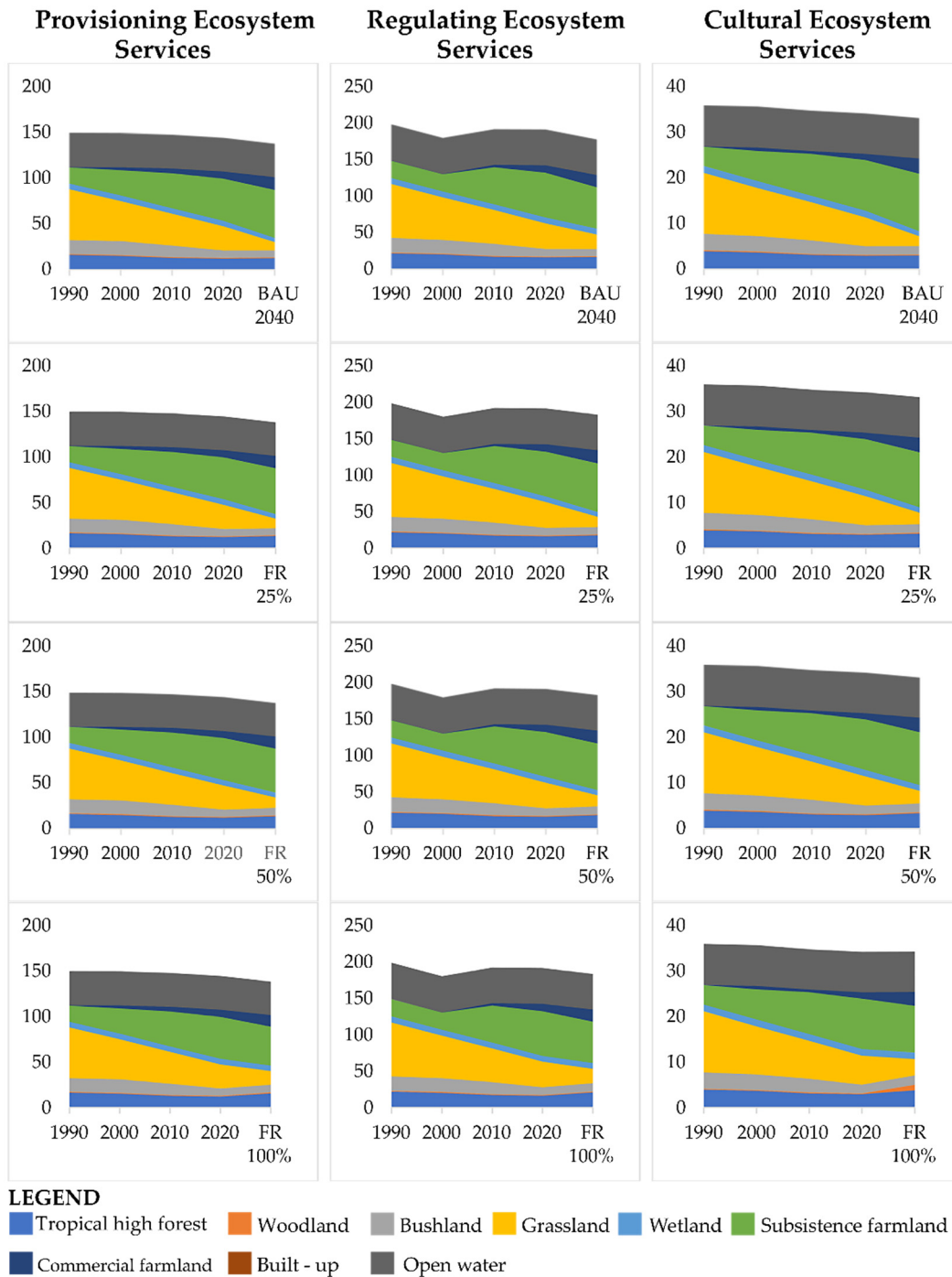
Figure 6. Historical and predicted ecosystem service potential for Budongo–Bugoma landscape.
