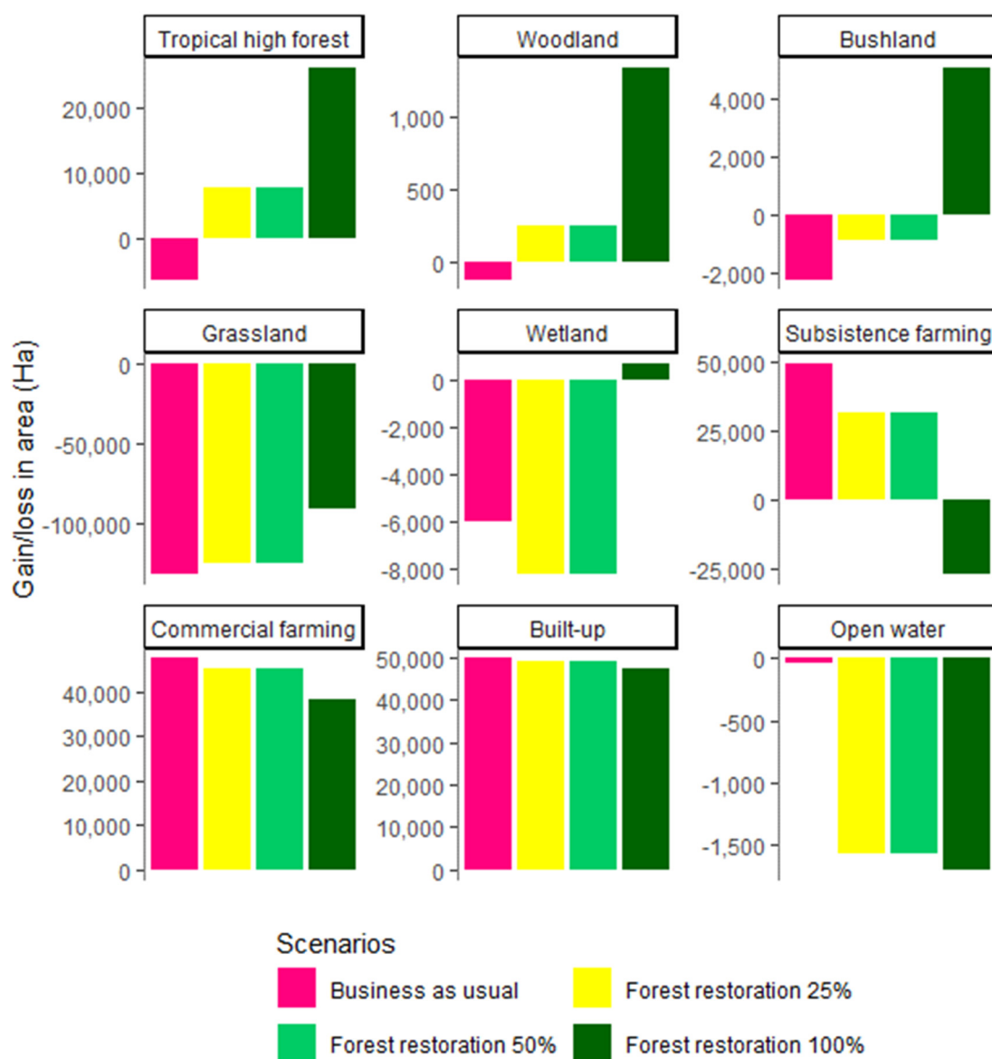
Figure 5. Predicted LULC gain and loss for Budongo–Bugoma landscape under different scenarios.
