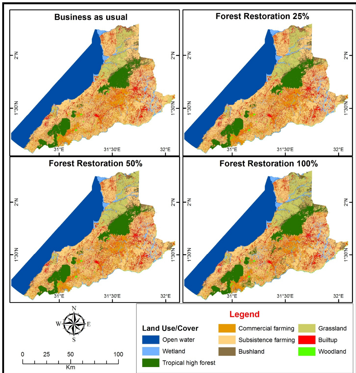
Figure 4. LULCC prediction maps for Budongo–Bugoma landscape under different scenarios in 2040.
