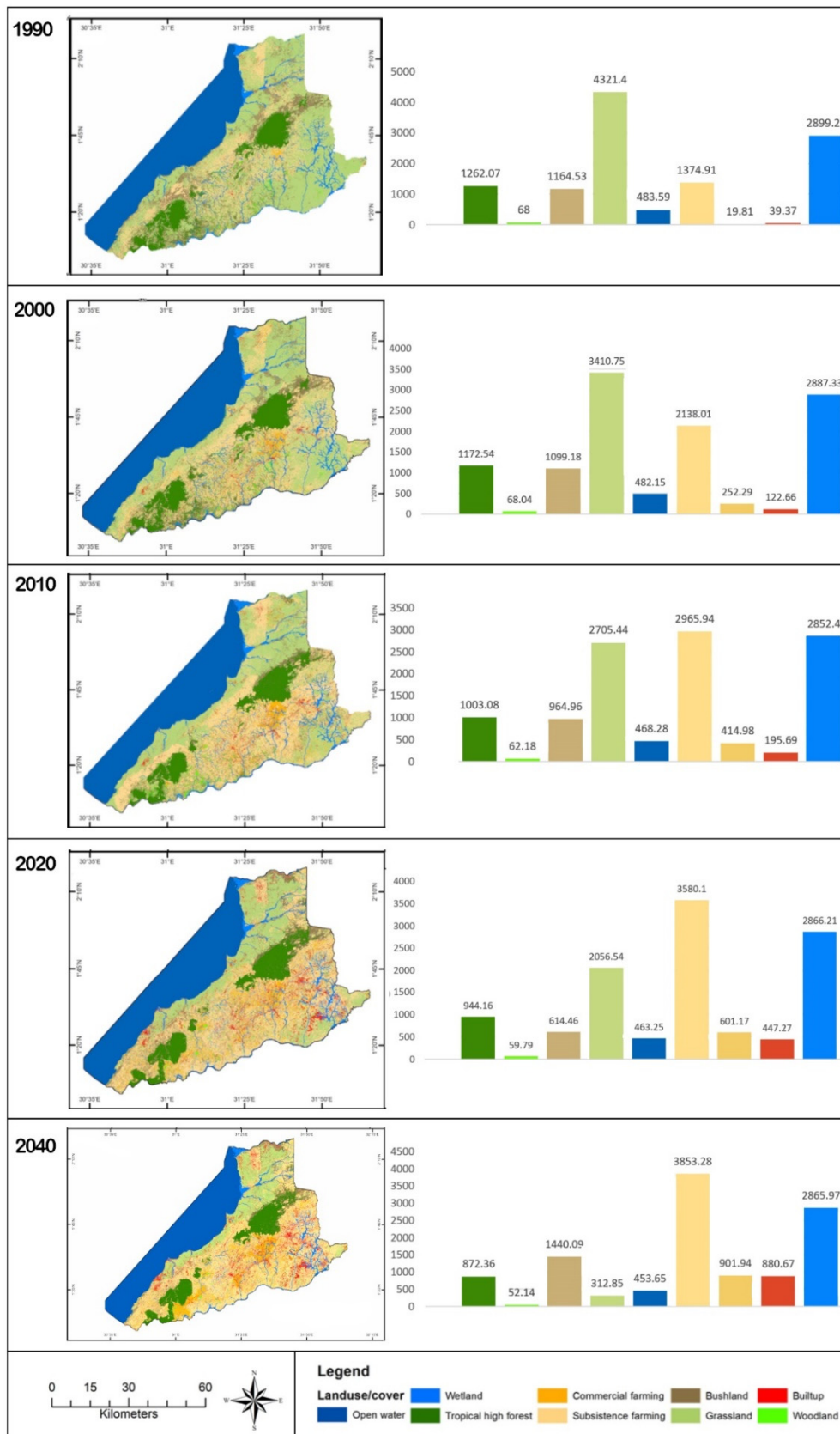
Figure A1. LULCC in the Budongo–Bugoma landscape using Landsat satellite imagery of single path and row (172/059).
