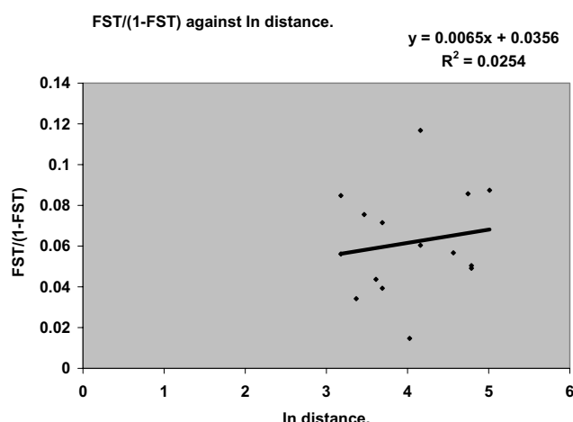
Figure 2 The effect of distance on population differentiation. The regression was made using F_{ST}/(1 - F_{ST}) against natural log (ln) separation distance. The equation describes best-fit regression line and shows little correlation between geographic location and degree of differentiation or genotype count.
