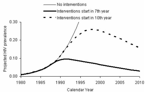
Fig. 2: Application of the model to parameter values for the case for Uganda
