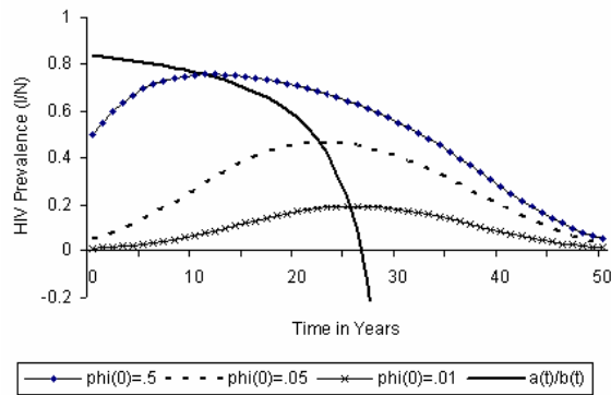
Fig. 1: Behavior of the non-autonomous logistic equation for prevalence \phi(t) = I(t)/N(t) with variable parameters
