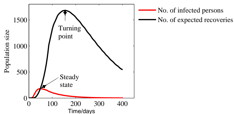
Fig. 5. Model (1) simulations for time series projection for the infected and expected recovered persons from COVID-19 in the presence of prevention and control measures.
