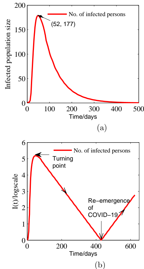
Fig. 6. (a) The number of infected persons as a function of time to linear scale. (b) The number of infected persons as a function of time to logarithm scale for R_{n0} = 0.46
