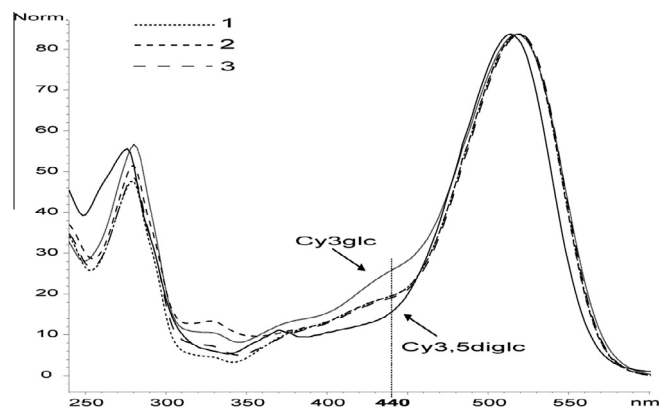
Fig. 1. UV-vis absorption spectra of compounds 1–3 on their flavylum cationic forms isolated from leaves of Hemigraphis colorata together with cyanidin 3- O -glucoside (Cy3glc) and cyanidin 3,5-di- O -glucoside (Cy3,5diglc) recorded on-line during HPLC analysis. The A_{440}/A_{vis-max} ratio has diagnostic value for identification of 5-methoxyanthocyanidins.
