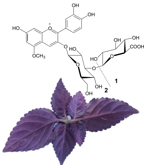
Fig. 2. Structures of 5- O -methylcyanidin 3- O -(3''-(β-glucuronopyranosyl)-β-glucopyranoside) ( 1 ) and 5- O -methylcyanidin 3- O -β-glucopyranoside ( 2 ) isolated from leaves of Hemigraphis colorata with purple abaxial surfaces.
