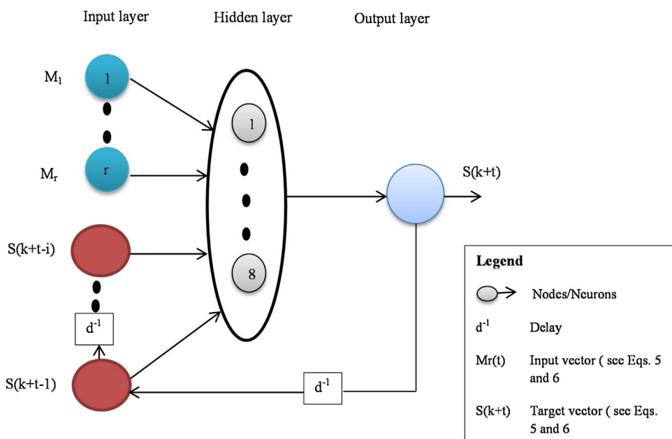
Fig. 2. Nonlinear autoregressive with exogenous input (NARX) model architecture showing the input, hidden and output layers and their flow directions.
