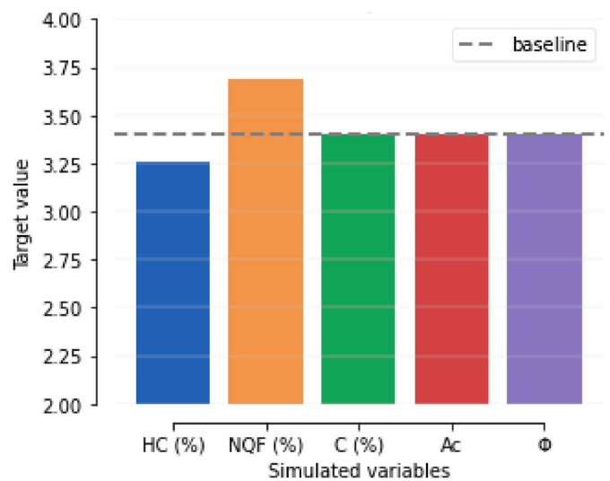
Fig. 16. Sensitivity analysis of the variables against the coefficient of uniformity model.
