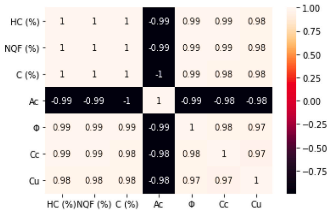
Fig. 3. Pearson's linear correlation of presented input and output variables.
