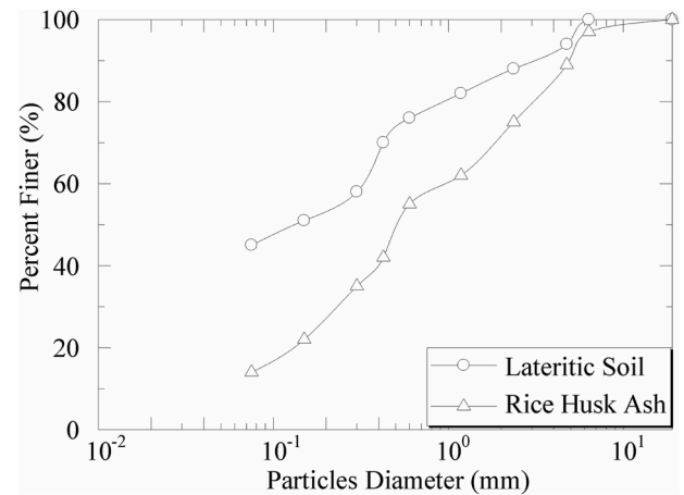
Fig. 6. Particle size distribution curve of clayey soil and rice husk ash.
