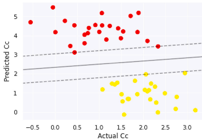
Fig. 9. The support vector model of coefficient of curvature.
