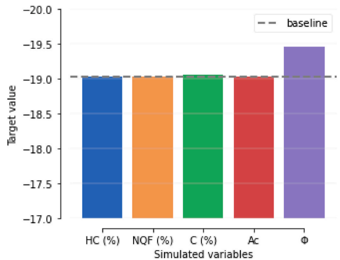
Fig. 15. Sensitivity analysis of the variables against the coefficient of curvature model.
