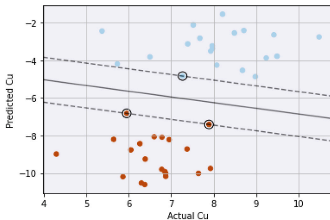
Fig. 10. The support vector model of coefficient of uniformity.
