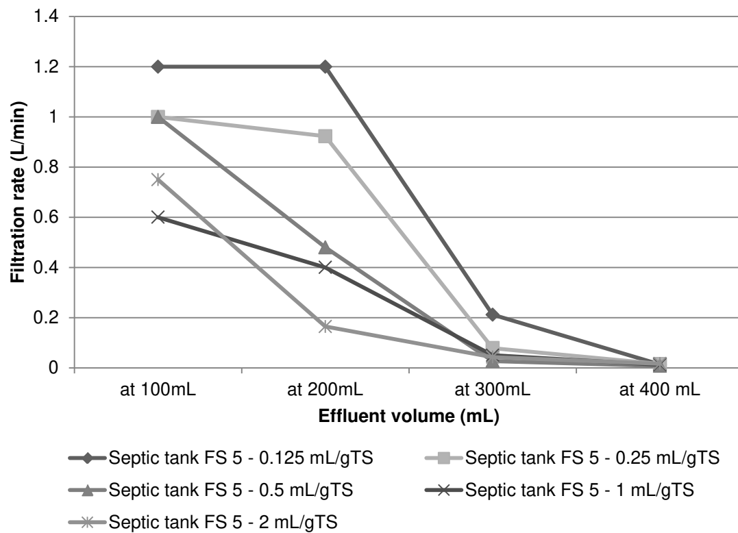
Figure 9: Filtration rate of conditioned septic tank FS in cone tests.
