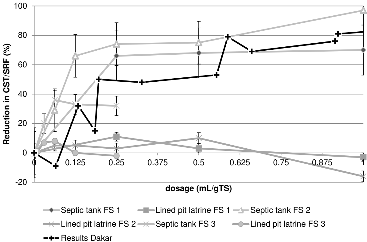
Figure 7: Reduction in CST by conditioning with chitosan in Kampala and Dakar (Gold et al., 2016). The number behind the sludge type refers to the repetition (see Table 1).
