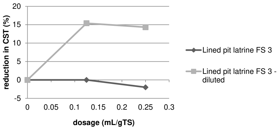
Figure 8: Reduction in CST for lined pit latrine FS, diluted and undiluted.
