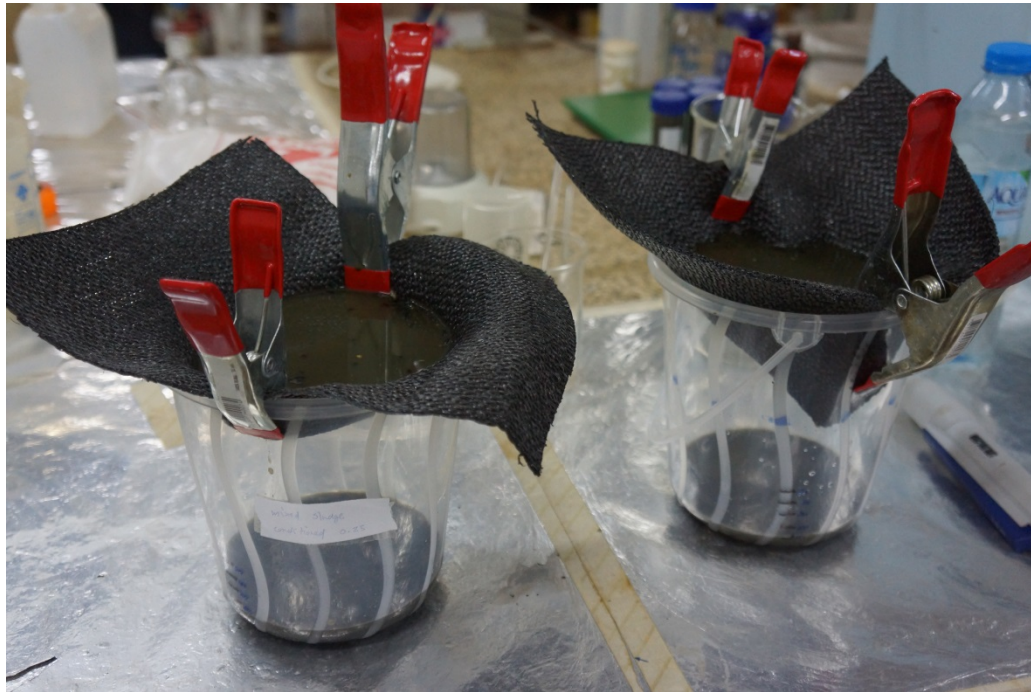
Figure 1: Experimental set up of geotextile cone tests
