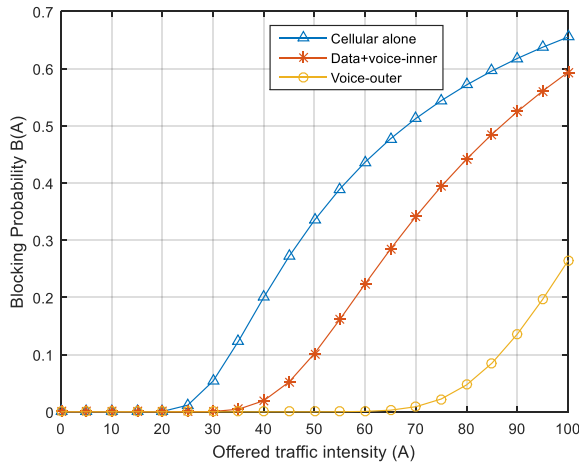
Fig.5: Blocking probability with borrowing
