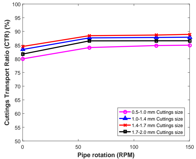
Figure 13: CTR vs. pipe rotation for different cutting sizes in horizontal hole for WBM and 8 ppb polypropylene beads
