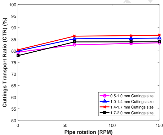
Figure 12: CTR vs. pipe rotation for different cutting sizes in horizontal hole for WBM and 6 ppb polypropylene beads
