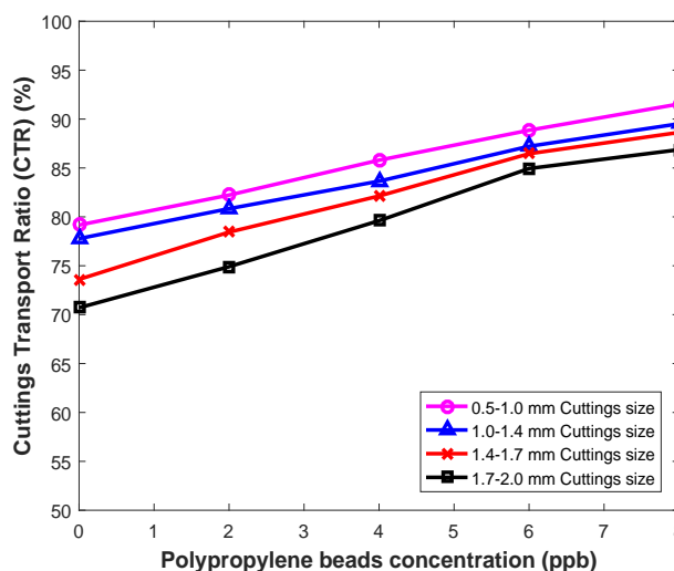
Figure 17: CTR of different cutting sizes with various polypropylene bead concentrations in horizontal hole
