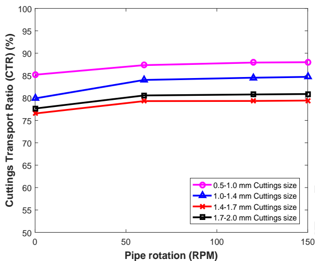
Figure 5: CTR vs. pipe rotation for different cutting sizes in vertical hole for WBM and 2 ppb polypropylene beads
