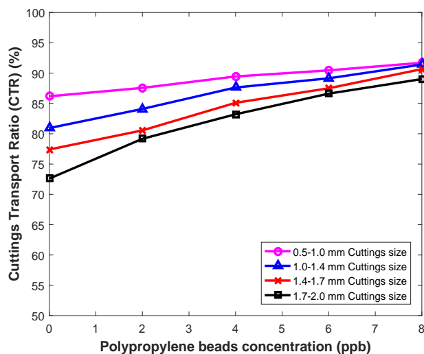
Figure 16: CTR of different cutting sizes with various polypropylene bead concentrations in vertical hole
