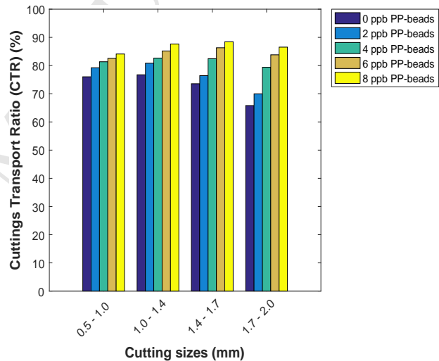
Figure 15: Cutting sizes in horizontal hole with pipe rotational speed of 60 rpm
