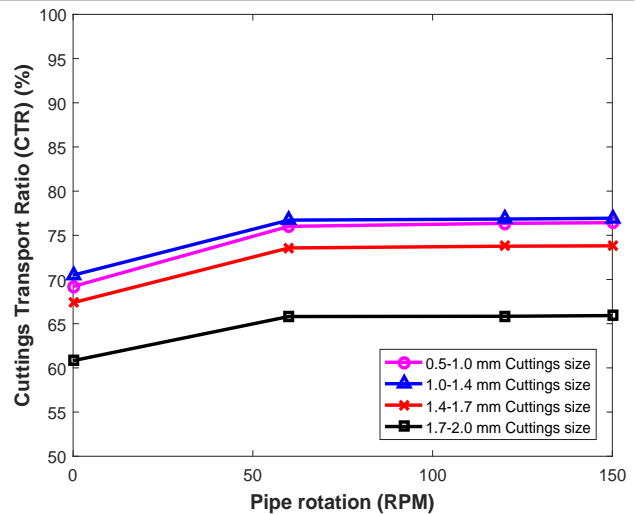
Figure 9: CTR vs. pipe rotation for different cutting sizes in horizontal hole for WBM
