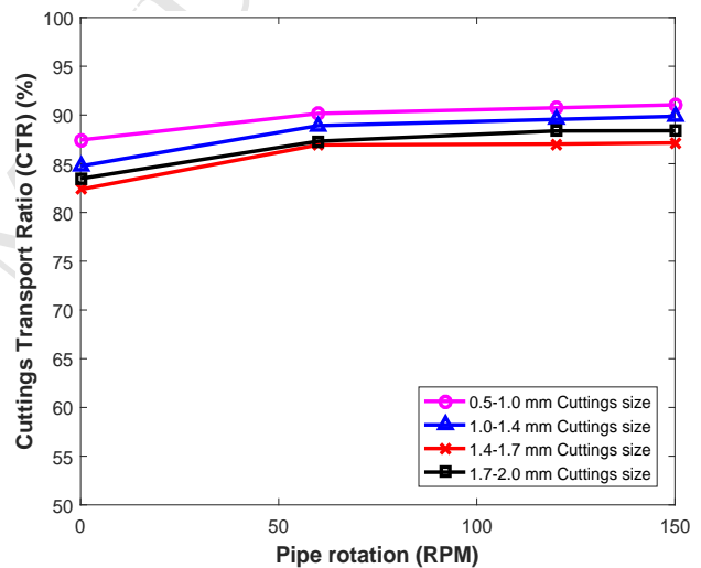
Figure 7: CTR vs. pipe rotation for different cutting sizes in vertical hole for WBM and 6 ppb polypropylene beads
