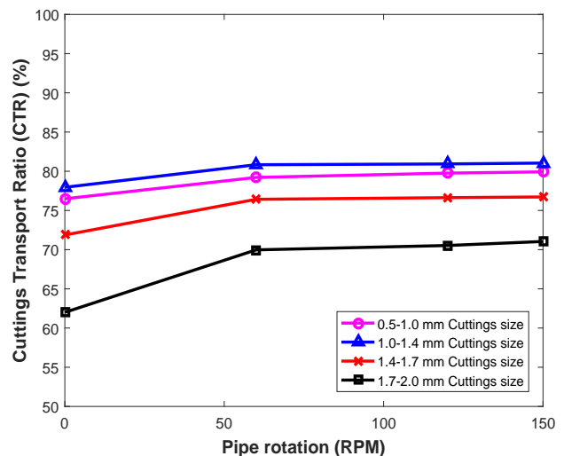
Figure 10: CTR vs. pipe rotation for different cutting sizes in horizontal hole for WBM and 2 ppb polypropylene beads
