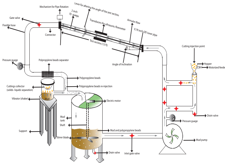
(a) Schematic of the flow-loop rig simulator
