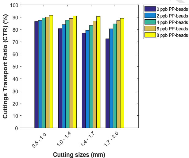
Figure 14: Cutting sizes in vertical hole with a pipe rotational speed of 60 rpm
