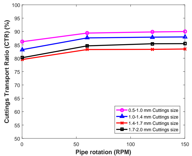
Figure 6: CTR vs. pipe rotation for different cutting sizes in vertical hole for WBM and 4 ppb polypropylene beads
