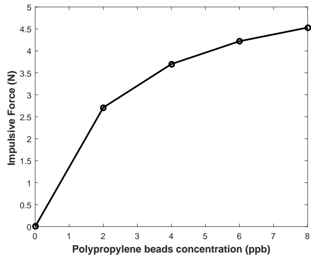
Figure 19: Impulsive force at various polypropylene bead concentrations
