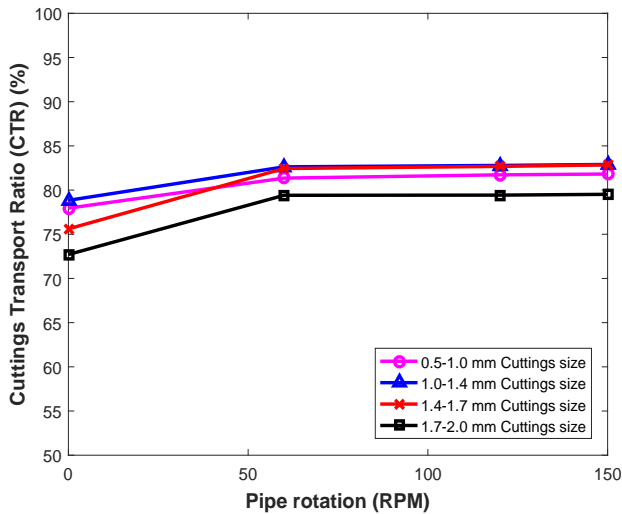
Figure 11: CTR vs. pipe rotation for different cutting sizes in horizontal hole for WBM and 4 ppb polypropylene beads
