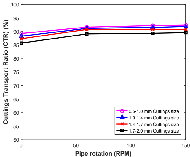
Figure 8: CTR vs. pipe rotation for different cutting sizes in vertical hole for WBM and 8 ppb polypropylene beads
