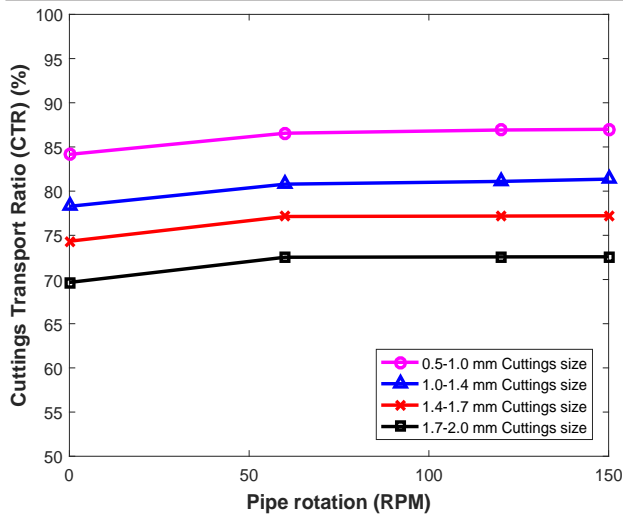
Figure 4: CTR vs. pipe rotation for different cutting sizes in vertical hole for WBM.
