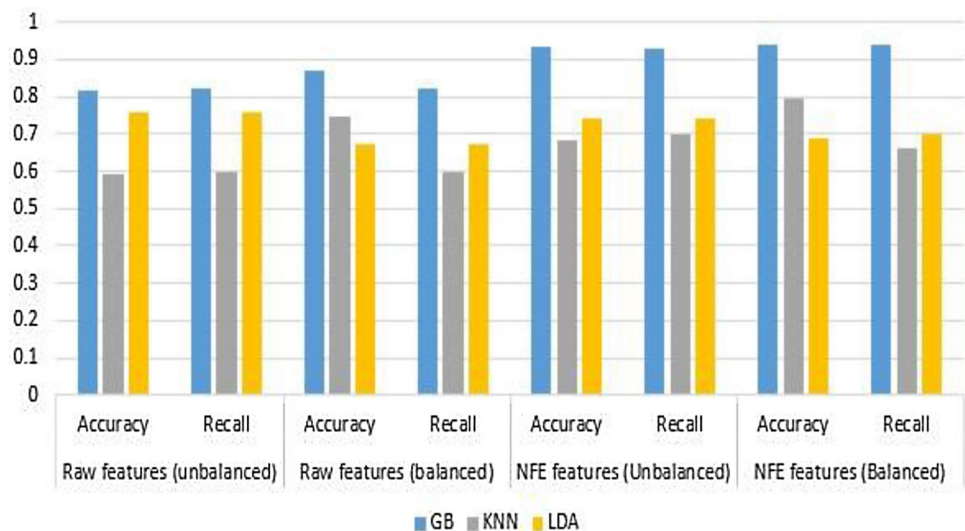
Fig. 8 Impact of NFE features on improving model classification performance
