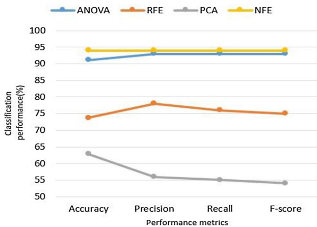
Fig. 9 Comparison between NFE, ANOVA, PCA, and RFE on feature selection performances
