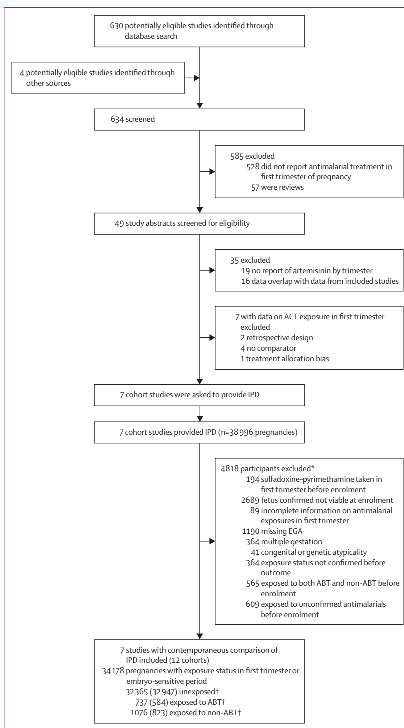
Figure 1: Study selection
