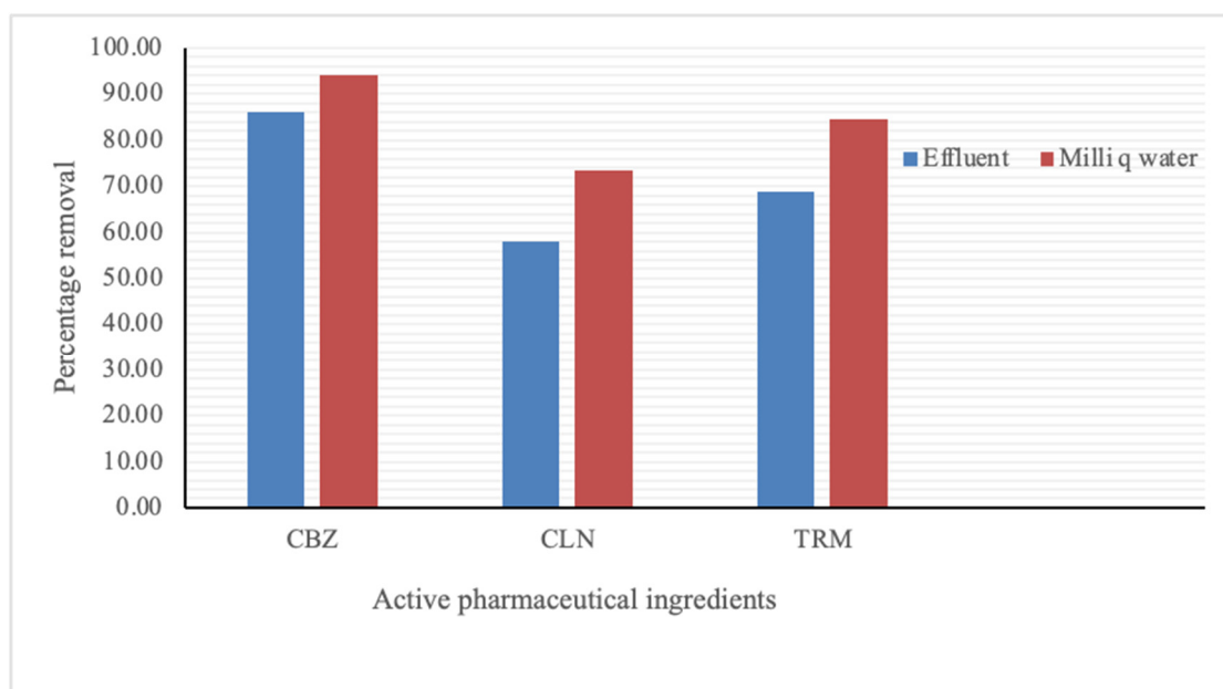
Figure 2. Percentage sequestration of APIs from affluent and Milli-Q water at equilibrium.
