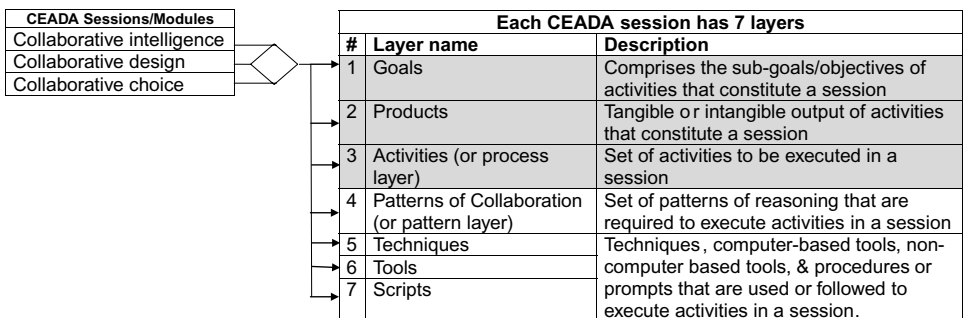
Fig. 5. Overview of CEADA and its composition.
