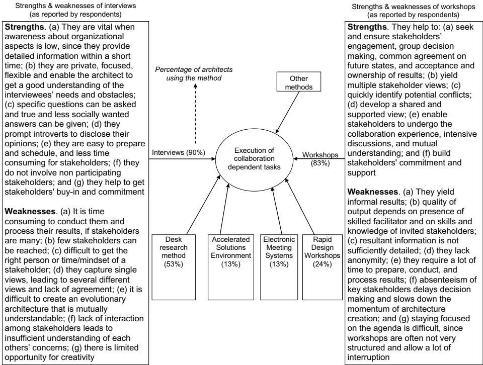
Fig. 3. Survey findings on methods used when executing collaborative tasks.
