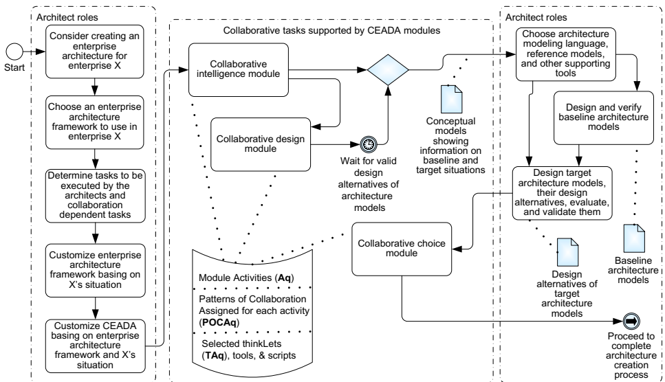
Fig. 23. Using CEADA along with an enterprise architecture framework.
