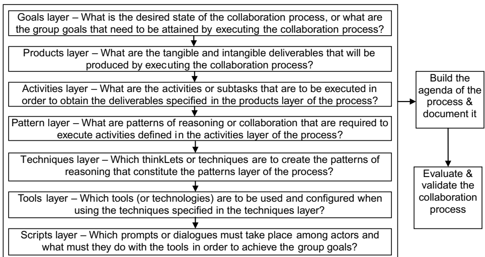
Fig. 4. Collaboration engineering approach (based on guidelines in Refs. 6, 7, 36 and 37).
