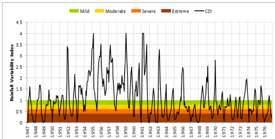
Fig. 2. Rainfall Variability Index for Namalu Station, Karamoja (1947-1976)
