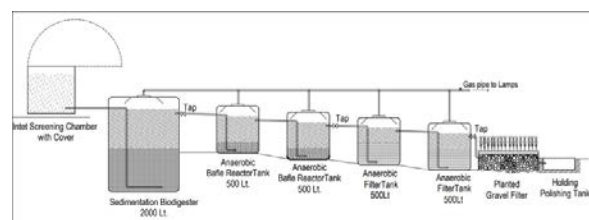
Figure 1: DEFASTS setup for primary, secondary and tertiary treatment
