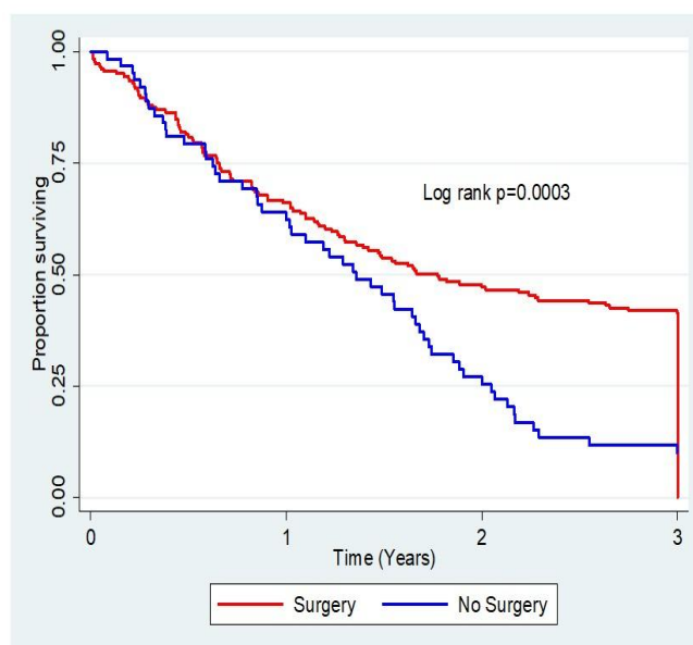
Fig. 2. Kaplan-Meier estimates of curative surgery alone, which has better survival rates than no surgery
