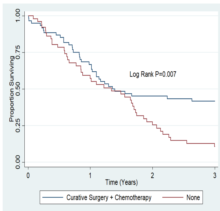
Fig. 5. Kaplan-Meier estimates showing better survival rates with curative surgery and adjuvant chemotherapy for select cases of stage II CRC and all stage III CRC patients
