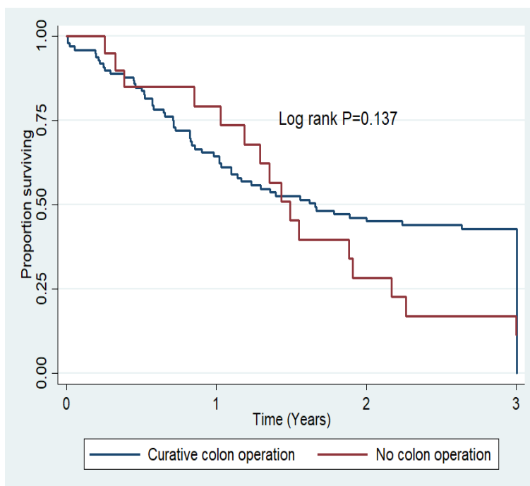
Fig. 4. Kaplan-Meier estimates of curative colon surgery alone showing a tendency towards better survival rates than no surgery
