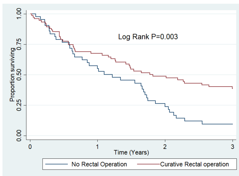
Fig. 3. Kaplan-Meier estimates of curative rectal surgery alone, which has better survival rates than no surgery
