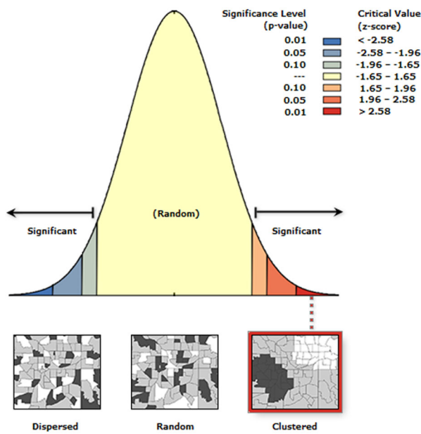
FIGURE 6 Graphical representation of acceptable regions for the measure of standard deviations and corresponding probabilities of Moran's metrics of spatial autocorrelation
