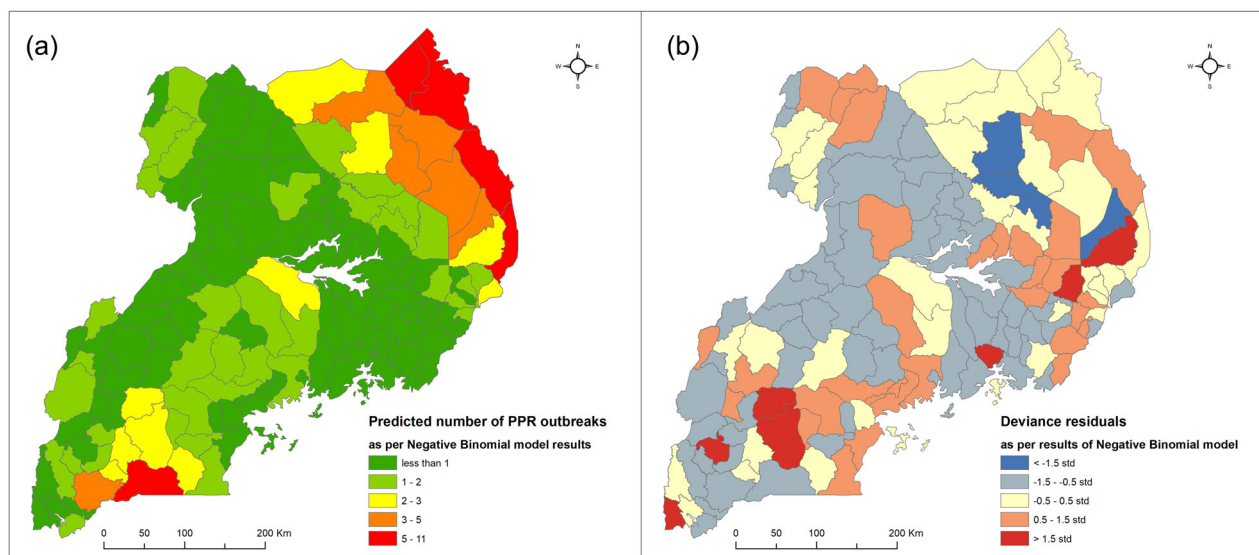
FIGURE 4 The predicted number of PPR outbreaks in Uganda as estimated by the negative binomial regression model and the distribution of the associated model residuals as visualised in ArcMap 10.7 software
