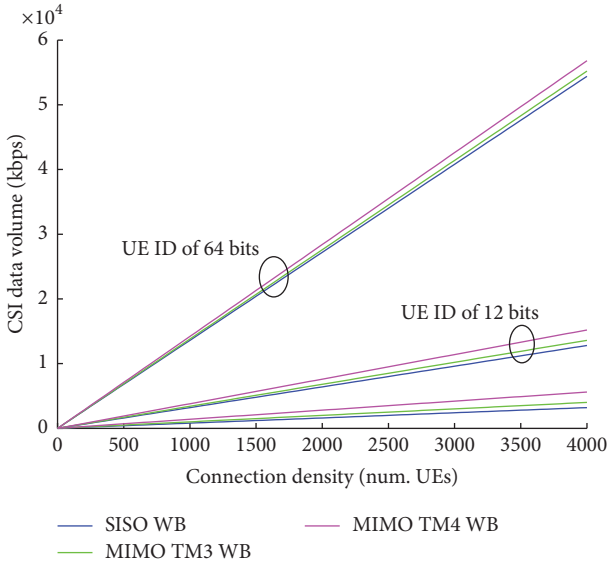
FIGURE 12: CSI data volume at CRR of 5 ms with LTE MIMO TM3, additional user identification bits, and increasing number of mobile users.
