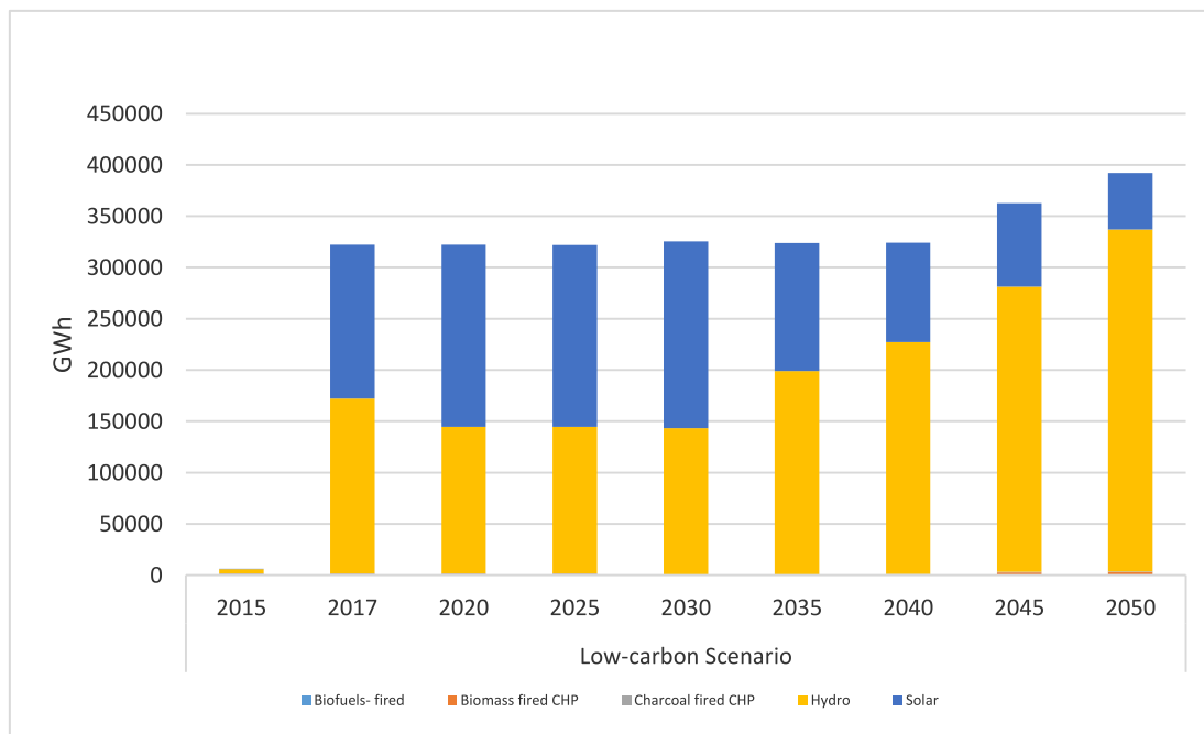
Figure 4. Electrical Power Production by Fuel type.
