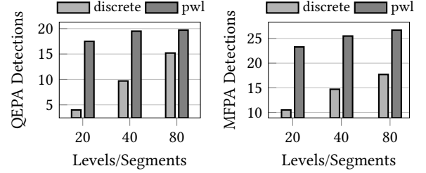
Figure 5: Improvement in solution quality of patrols planned for the QEPA and MFPA, using MILP (\mathcal{P}_2) compared to previous work using discrete levels of patrol effort. The utility is measured in number of predicted detected attacks.
