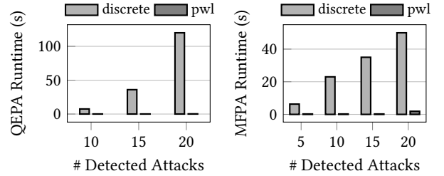
Figure 6: Improvement in runtime for computing patrols for QEPA and MFPA, using MILP (\mathcal{P}_2) compared to previous work using discrete levels of patrol effort for comparable solution quality, measured in predicted number of detected attacks. Results are averaged over 20 trials.
