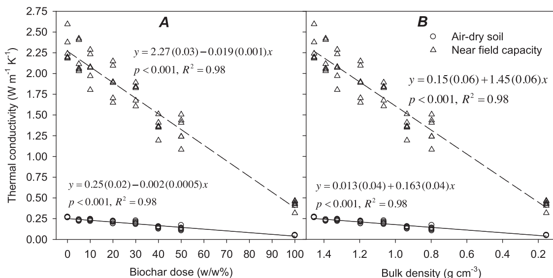
Fig. 4. Thermal conductivity of Mkushi soil mixed with pigeon pea BC as a function of BC dose (A) and bulk density (B).
