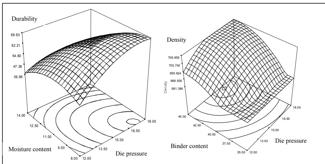
Figure 2: Response surface and contour plots of the durability response
