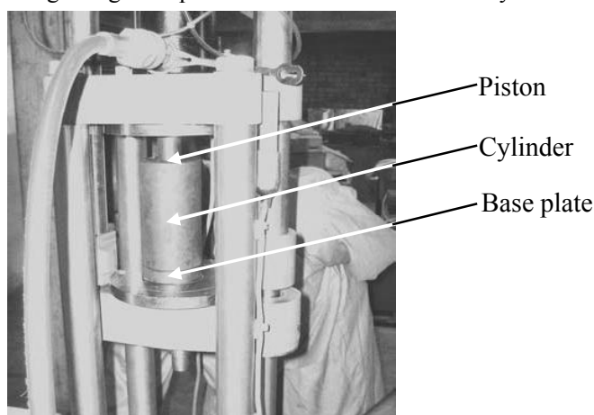
Figure 1: Compression of briquette samples using a compression testing machine
